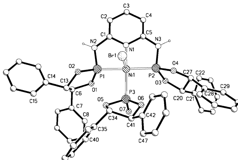
Figure 1. Structural view of [\text{Ni}(\text{PNP-HBz})\{\kappa^1(\text{P})\text{-HBz-P=O}\}\text{Br}] ( 2i-CH 3 OH ) (second independent Ni complex, C-bonded H atoms and CH 3 OH omitted for clarity). Selected bond lengths [Å] and bond angles [°]: Ni(1)–N(1) 1.913(8), Ni(1)–P(1) 2.144(3), Ni(1)–P(2) 2.114(3), Ni(1)–P(3) 2.132(6), Ni(1)–Br(1) 2.535(4); P(1)–Ni(1)–P(2) 157.6(3), N(1)–Ni(1)–P(3) 163.6(4), Br(1)–Ni(1)–N(1) 97.1(4), Br(1)–Ni(1)–P(1) 98.7(2), Br(1)–Ni(1)–P(2) 101.8(2), Br(1)–Ni(1)–P(3) 99.2(2).
