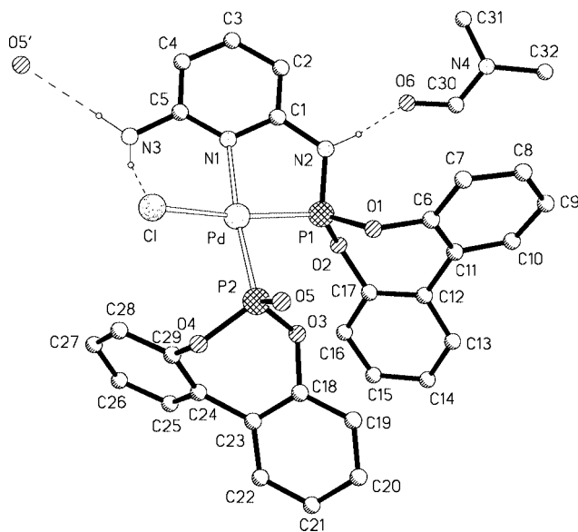
Figure 2. Structural view of [\text{Pd}\{\kappa^2(\text{P},\text{N})\text{-NH}_2\text{-PN-BIPOL}\}\{\kappa^1(\text{P})\text{-BIPOL-P=O}\}\text{Cl}]\cdot\text{DMF} ( 4 ·DMF) (C-bonded H atoms omitted for clarity). Selected bond lengths [Å] and bond angles [°]: Pd–N(1) 2.171(2), Pd–P(1) 2.1787(5), Pd–P(2) 2.2276(6), Pd–Cl 2.3505(5); P(1)–Pd–P(2) 91.78(2), Cl–Pd–P(2) 86.76(2), N(1)–Pd–P(2) 173.51(5), Cl–Pd–P(1) 165.39(2).
